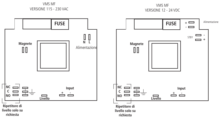
Fig. 38. Schema circuito VMS MF / VMSA MF
